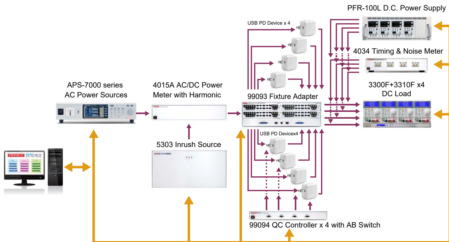
6050-4-D-X 4 Channel with AB Switch Test System Configuration
