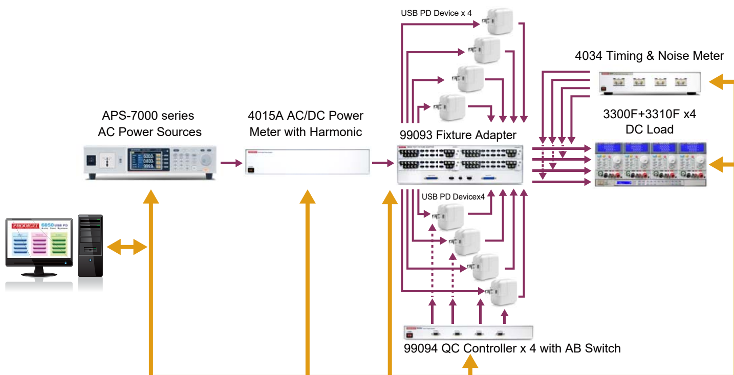
6050-4-C-X 4 Channel with AB Switch Test System Configuration
