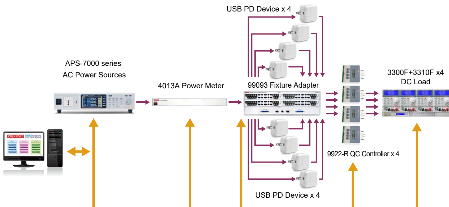
6050-4-A-X 4 Channel with AB Switch Test System Configuration
