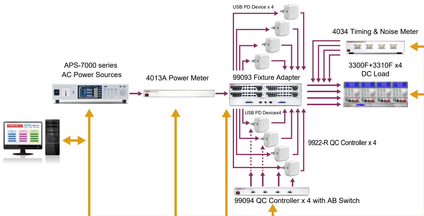
6050-4-B-X 4 Channel with AB Switch Test System Configuration
