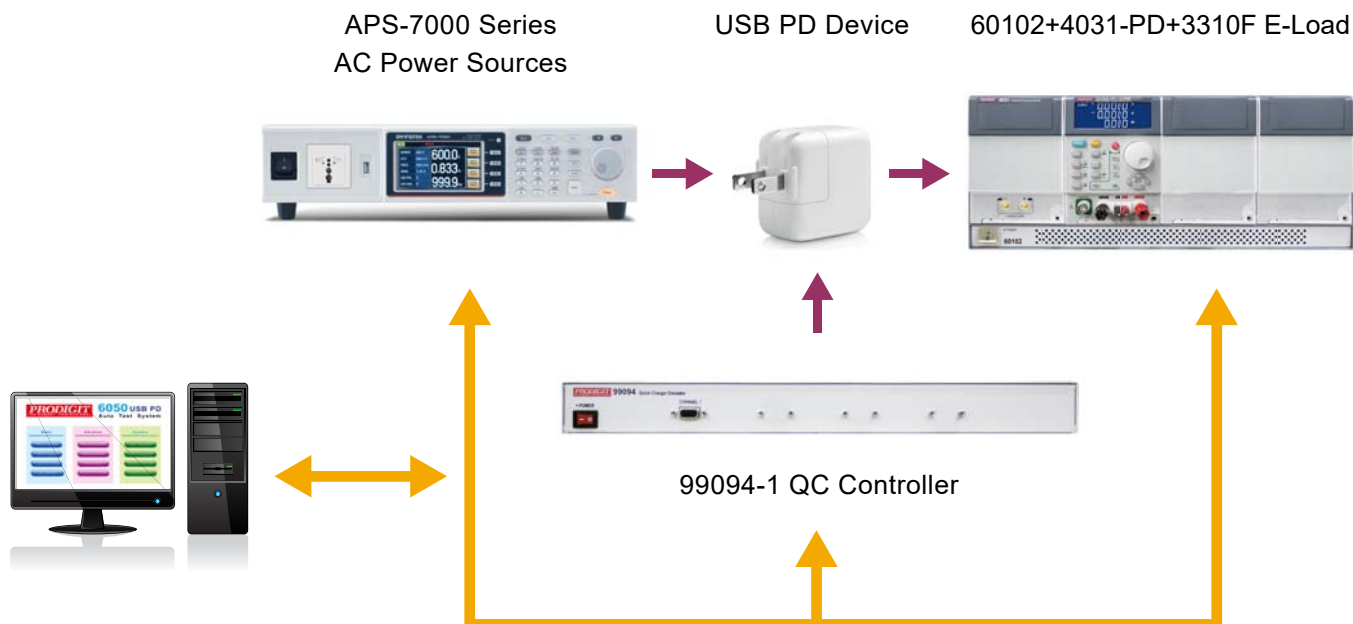
6050-1-B Single Channel Test System Configuration
