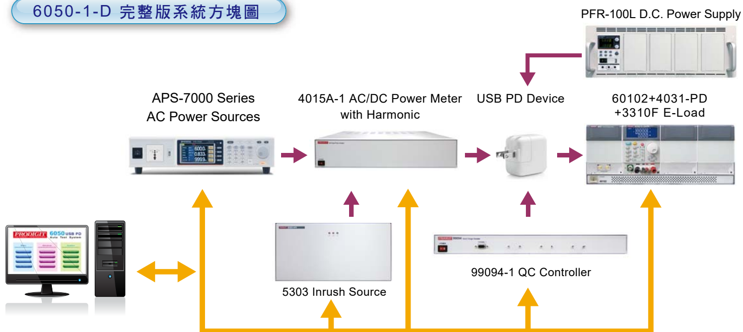
6050-1-D Single Channel Test System Configuration
